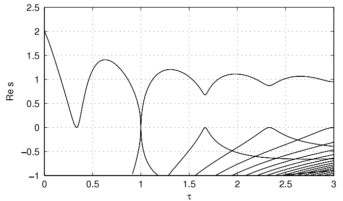
Fig. 2. The real part vs \tau . The touching points to the right of the \tau_0 = 1 are from below. This corresponds to case 1.
