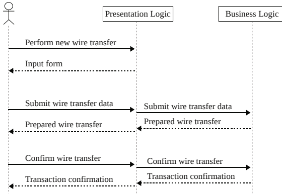
(a) Original application
