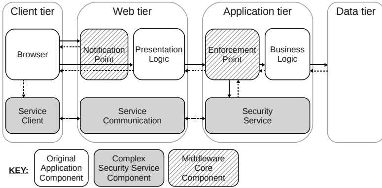
Fig. 2. The high-level architecture of the security middleware in a four tier web architecture
