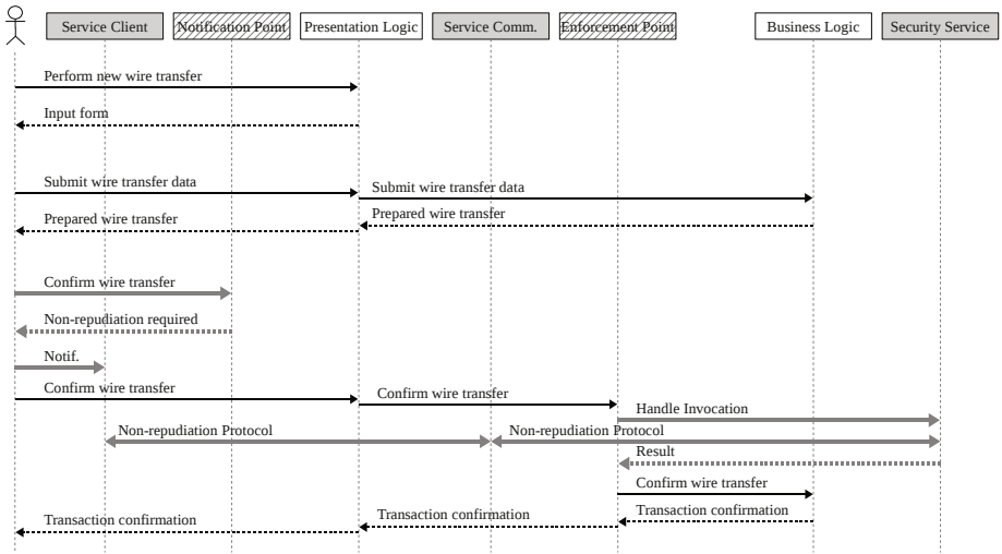
(b) Application with an integrated non-repudiation service
