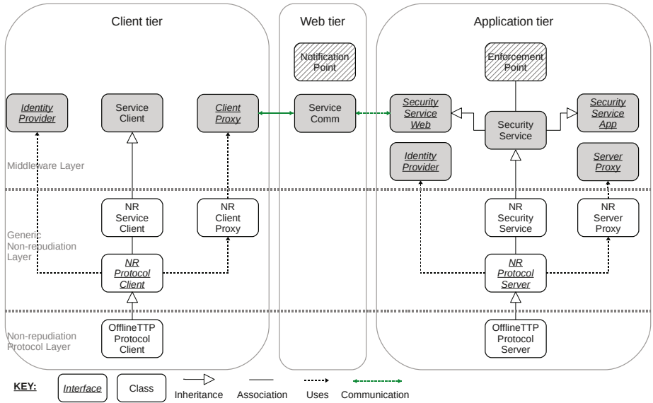
Fig. 4. The detailed design of the security middleware and a specific complex security service (non-repudiation)
