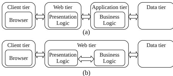
Fig. 1. (a) A typical enterprise web architecture with four distinct tiers. (b) A lightweight web architecture with business logic embedded in the web tier.
