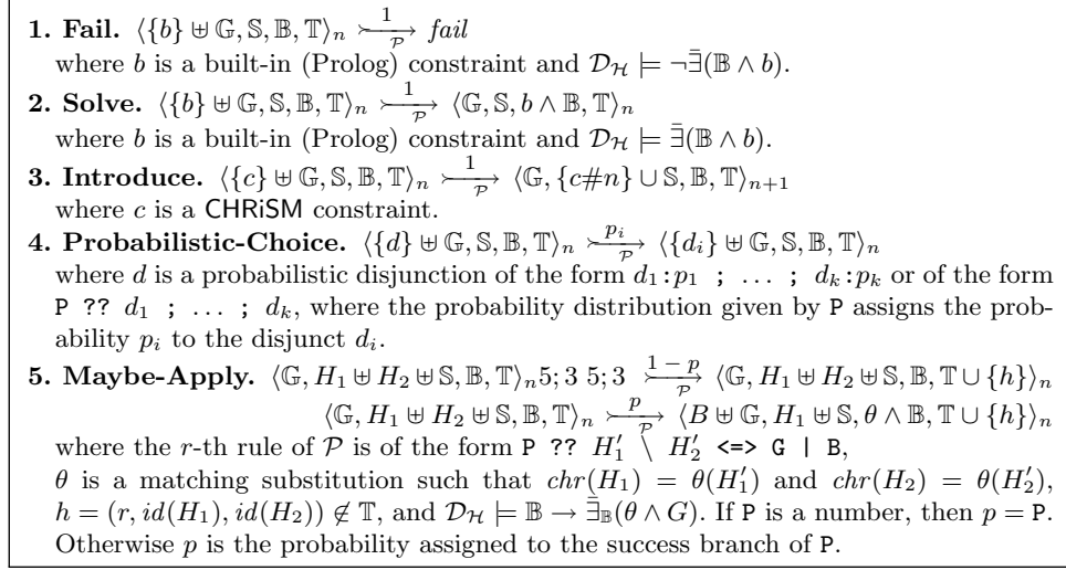
Fig. 1. Transition relation \xrightarrow{p} of the abstract operational semantics \omega_i^{??} of CHRiSM.
